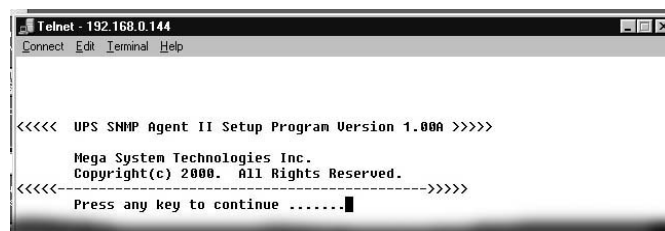
Fig.40 Telnet Connection
