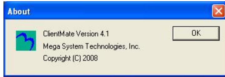
Fig.47 ClientMate>About
